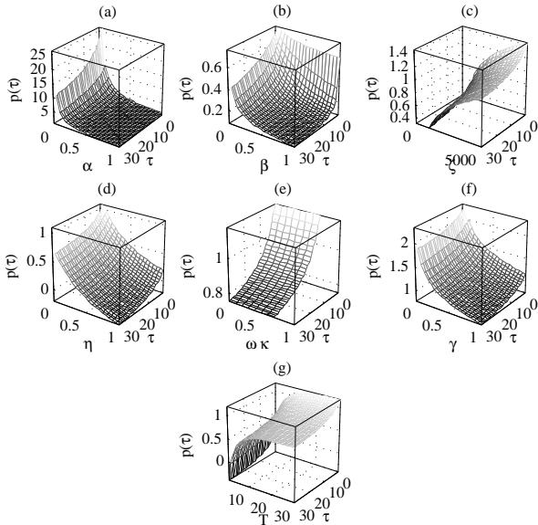
Figure 2: The impact of model parameters on the guaranteed selling prices: \alpha , \beta , \zeta , \eta are defined in Eqs. (4) & (5); \omega\kappa is the expected size of penalty; \gamma is the percentage of estimated future impressions to sell in advanced; T is the length of guaranteed selling period; \tau is the remaining time to the delivery date; p(\tau) is the guaranteed selling price at \tau .
