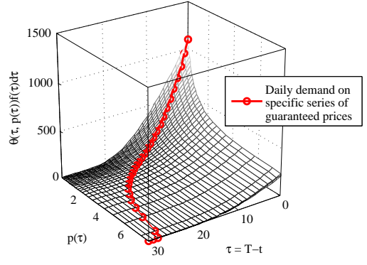
Figure 8: A numerical example of demand surface for guaranteed impressions of an ad slot, where \theta(\tau, p(\tau))f(\tau)d\tau represents the number of advertisers who will buy guaranteed impressions at p(\tau) and in [\tau, \tau + d\tau] ; other parameters are \alpha = 1.85 ; \beta = 0.01 ; \zeta = 2000 ; \eta = 0.01 ; T = 30 .
